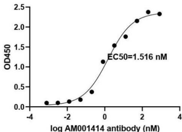
Fig.1 SARS-CoV-2 Spike RBD protein was coated onto microtiter plates at 0.5 µg/mL and then incubated with a dilution series of Spike S1 Neutralizing Antibody (SARS-CoV-2) (Clone: 414-1). Bound antibodies were detected with anti-human IgG conjugated to horseradish peroxidase (HRP) followed by incubation with HRP Substrate and then measuring the resulting absorbance at 450 nm.
