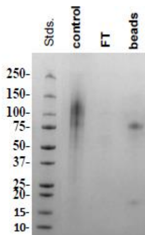
Biotin-Avidin Pulldown
