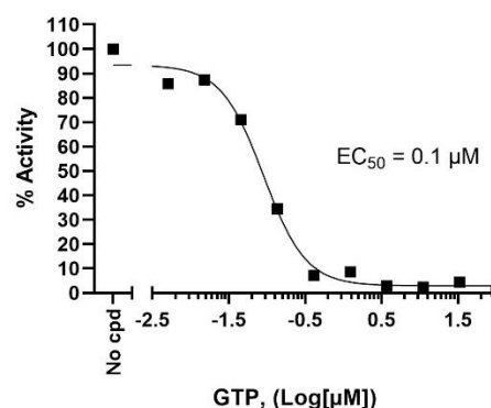
KRAS (G12V), GDP-Loaded Activity
