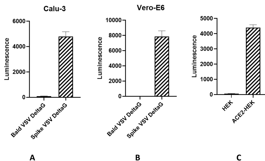
Figure 1. Transduction of Calu-3, Vero-E6, and ACE2-HEK293 cells.
