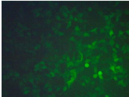
Figure 2. Transduction of HEK293 cells using eGFP lentivirus. Approximately 5,000 cells/well of HEK293 cells were transduced with 2 \mu l/well of eGFP lentivirus. After 66 hours of transduction, the expression of eGFP in the target cells was observed under a fluorescence microscope.
