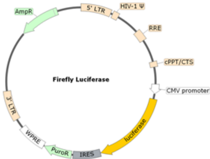
Figure 1. Schematic of the lenti-vector used to introduce the luciferase reporter in Spike (BA.2.86, Omicron Variant) (SARS-CoV-2) Pseudotyped Lentivirus (Luciferase Reporter).
