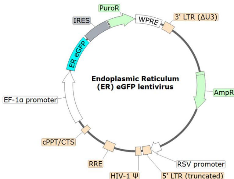
Figure 1. Schematic of the lenti-vector used to generate the Endoplasmic Reticulum (ER) eGFP Lentivirus.
