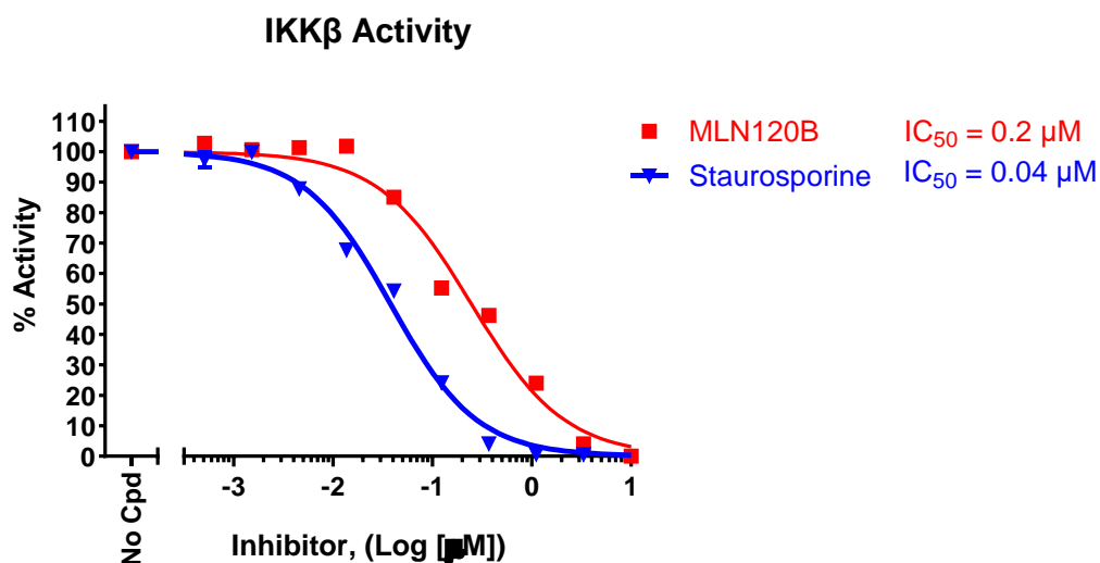
Figure 1: Inhibition of IKKβ kinase activity by the inhibitors MLN120B and Staurosporine. IKKβ kinase activity was measured in the presence of increasing concentrations of MLN120B (#82605) or Staurosporine (#27002). The “Blank” value was subtracted from all other values. Results are expressed as the percent of control (kinase activity in the absence of inhibitor, set at 100%).
