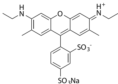
Figure 1. Structure of Sulforhodamine G.
