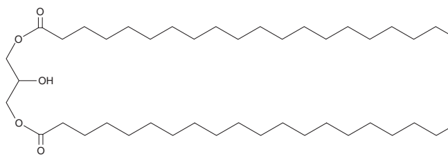
Unspecified isomer
