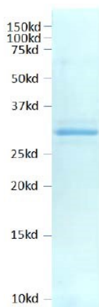
SDS-PAGE: purified VP1 protein of FMDV (strain A24 Cruzeiro)
