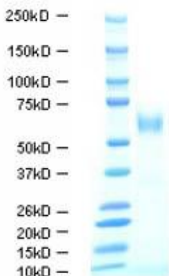
SDS-PAGE: purified HA1 (H1N1)(A//Puerto Rico/8/1934) protein
