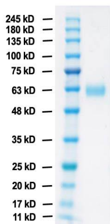
SDS-PAGE: purified HA1 (H4N6)(A/mallard/Ohio/657/2002) protein
