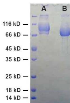
SDS-PAGE: purified HA (B/Brisbane/60/2008)(aa 16-546) protein A , non-reducing condition; B , reducing condition
