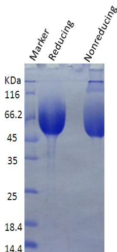
SDS-PAGE: purified HA1 (H3N2)(A/Switzerland/9715293/2013) protein.
