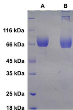
SDS-PAGE: purified HA (A/California/07/2009/H1N1) (aa 18-529) protein; A , reducing condition; B , non-reducing condition.
