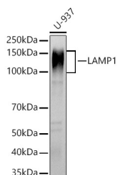
Western blot analysis of U-937 using LAMP1 Polyclonal Antibody at 1:1000 dilution. Observed Mw: 90-120kDa Calculated Mw: 38kDa/44kDa
