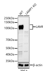
Western blot analysis of extracts from wild type (WT) and LAMP1 knockout (KO) HeLa cells using LAMP1 Polyclonal Antibody at 1:1000 dilution.
