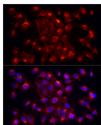
Immunofluorescence analysis of HeLa cells using [KO Validated] LAMP1 Polyclonal Antibody at dilution of 1:20 (40x lens). Blue: DAPI for nuclear staining.
