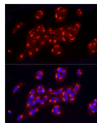
Immunofluorescence analysis of U2OS cells using [KO Validated] LAMP1 Polyclonal Antibody at dilution of 1:20 (40x lens). Blue: DAPI for nuclear staining.
