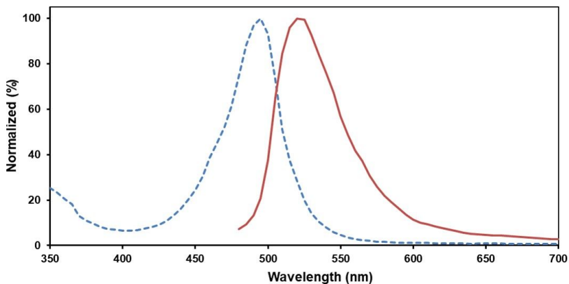
AF488 Excitation and Emission Spectra
