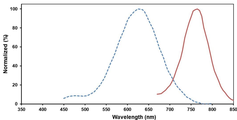
ER780 Excitation and Emission Spectra
