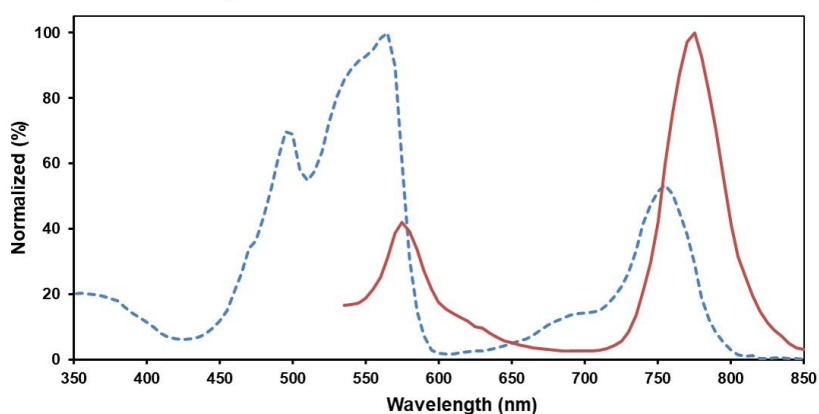
PE/Cyanine7 Excitation and Emission Spectra
