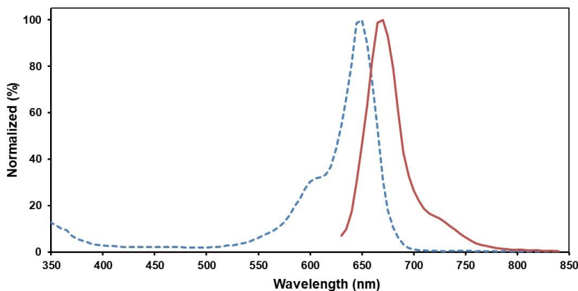
AF647 Excitation and Emission Spectra
