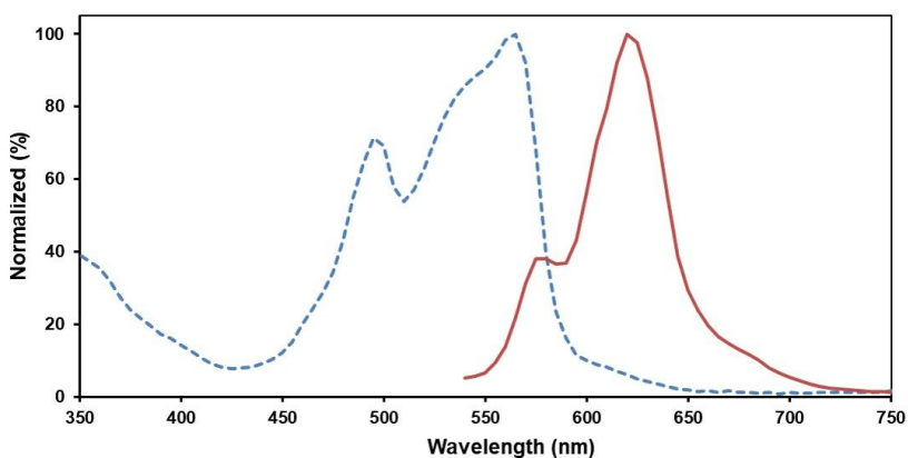
PE/TR Excitation and Emission Spectra
