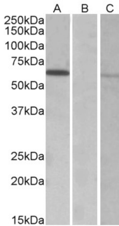
HEK293 lysate (10 \mu g protein in RIPA buffer) over expressing Human MKRN1 with DYKDDDDK tag probed with EB10898 (0.3 \mu g/ml) in Lane A and probed with anti- DYKDDDDK Tag (1/1000) in lane C. Mock-transfected HEK293 probed with EB10898 (1 \mu g/ml) in Lane B. Primary incubations were for 1 hour. Detected by chemiluminescence.
