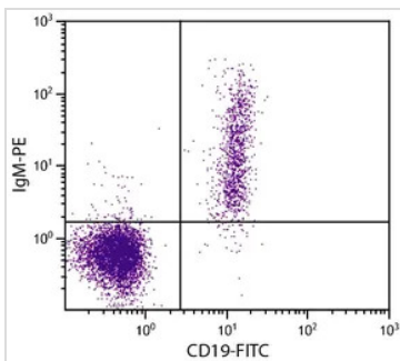
GTX04120-08 FACS Image
