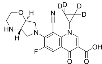
HCl
