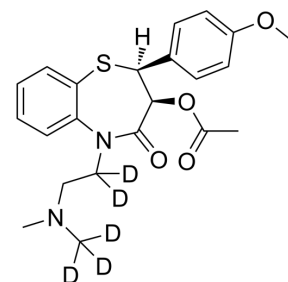
HCl
