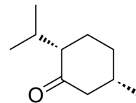
Relative stereochemistry
