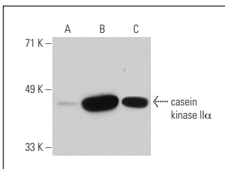
casein kinase II \alpha (1A09): sc-12738. Western blot analysis of casein kinase II \alpha expression in non-transfected: sc-117752 (A), human casein kinase II \alpha transfected: sc-116435 (B) and human casein kinase II \alpha transfected: sc-117423 (C) 293T whole cell lysates.
