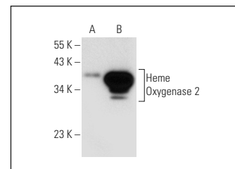
Heme Oxygenase 2/3 (B-4): sc-166299. Western blot analysis of Heme Oxygenase 2 expression in non-transfected: sc-117752 (A) and mouse Heme Oxygenase 2 transfected: sc-120746 (B) 293T whole cell lysates.
