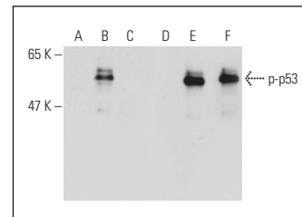
Western blot analysis of p53 phosphorylation in non-transfected: sc-117752 (A, D), untreated human p53 transfected: sc-158802 (B, E) and lambda protein phosphatase treated human p53 transfected: sc-158802 (C, F) 293T whole cell lysates. Antibodies tested include p-p53 (59.Ser 315): sc-135772 (A, B, C) and p53 (Pab 240): sc-99 (D, E, F).
