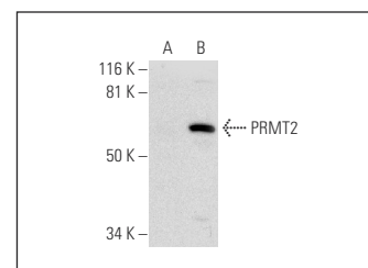
PRMT2 (B-11): sc-393254. Western blot analysis of PRMT2 expression in non-transfected: sc-117752 (A) and human PRMT2 transfected: sc-172533 (B) 293T whole cell lysates.
