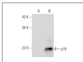
p18 (DCS-118): sc-56332. Western blot analysis of p18 expression in non-transfected: sc-117752 (A) and human p18 transfected: sc-174498 (B) 293T whole cell lysates.
