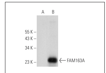
FAM163A (G-12): sc-393821. Western blot analysis of FAM163A expression in non-transfected: sc-117752 (A) and human FAM163A transfected: sc-175533 (B) 293T whole cell lysates.
